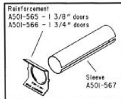
37-001 Reinforcement Kit
