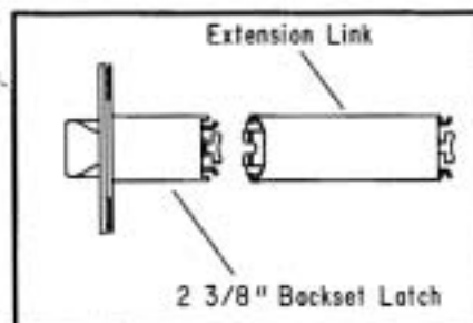
41-005 5" Extension Link
