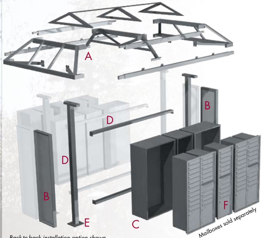
Back-to-back installation option shown installed behind standard layout with gable peak roof option
