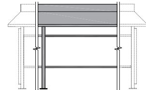
VAR4E(O) End-to-End or VAR4BE(O) Back-to-Back/ End-to-End Mid-Section
